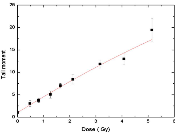
Figure 5. Variation of OTM with dose for human peripheral blood cells after 8 M eV Pulsed electron beam irradiation.
