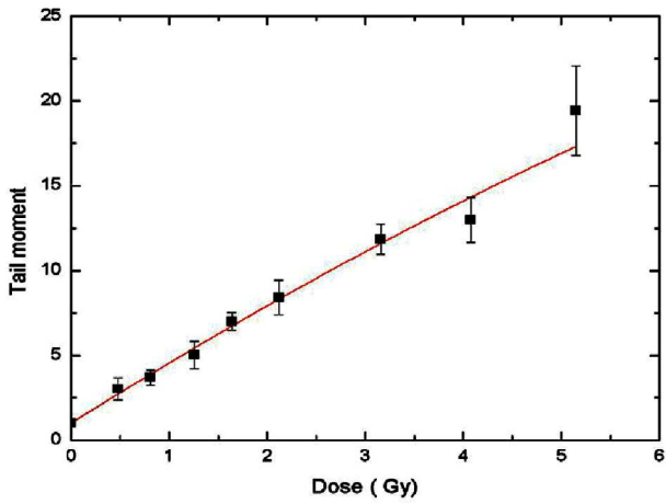
Figure 4. Variation of Tail Moment with dose for human peripheral blood cells after 8 M eV Pulsed electron beam irradiation.
