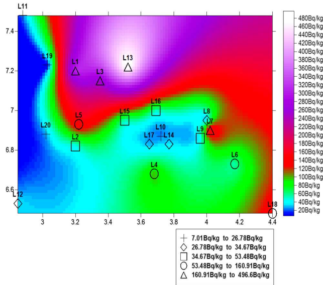
Figure 3. The image map of ^{232}\text{Th} activity concentrations for the study area.
