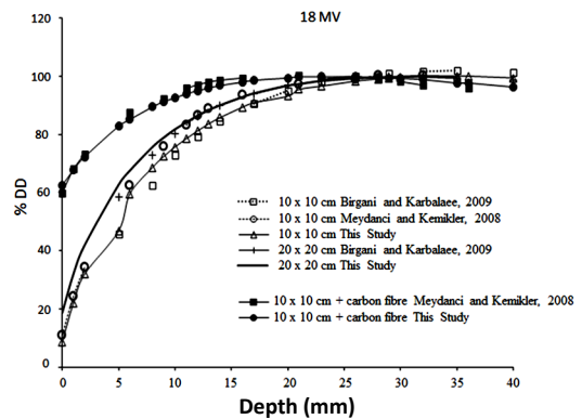
Figure 4. Percentage depth dose (%DD) curves with and without the carbon fiber tabletop for various field sizes for an 18MV photon beam.
