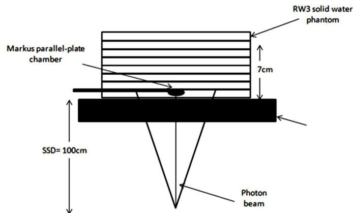
Figure 2. Experimental setup for measurement of the dose to the surface and buildup region for a carbon-fiber tabletop ( 180^\circ ).
