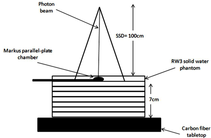
Figure 1. Experimental setup for measurement of the dose to the surface and buildup region for an open beam ( 0^\circ ).
