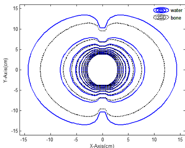
Figure 7. A comparison between the isodose distributions in bone and water.
