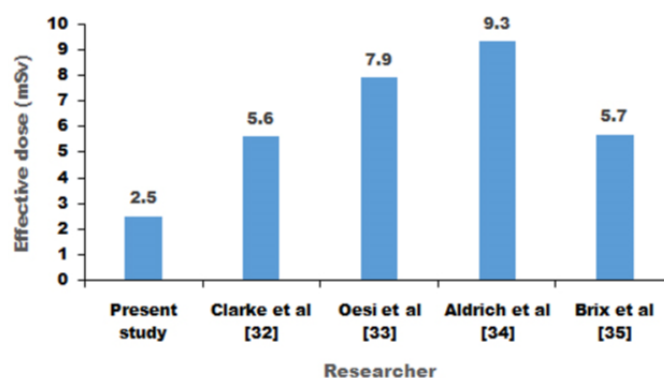
Figure 2. Comparison of estimated effective dose in adult chest computed tomography examination obtained using a Rando phantom and thermoluminescent dosimeters with values in literature. The present study was conducted using a Phillips Brilliance 64-slice CT scanner computed tomography (CT) scanner fitted with fitted with improved Dose Optimization Software (Automatic Exposure Control (AEC)). Comparative estimates were much higher since older models of CT scanners were used. These were not installed with AEC software that automatically reduces tube current in accordance to patient size.
