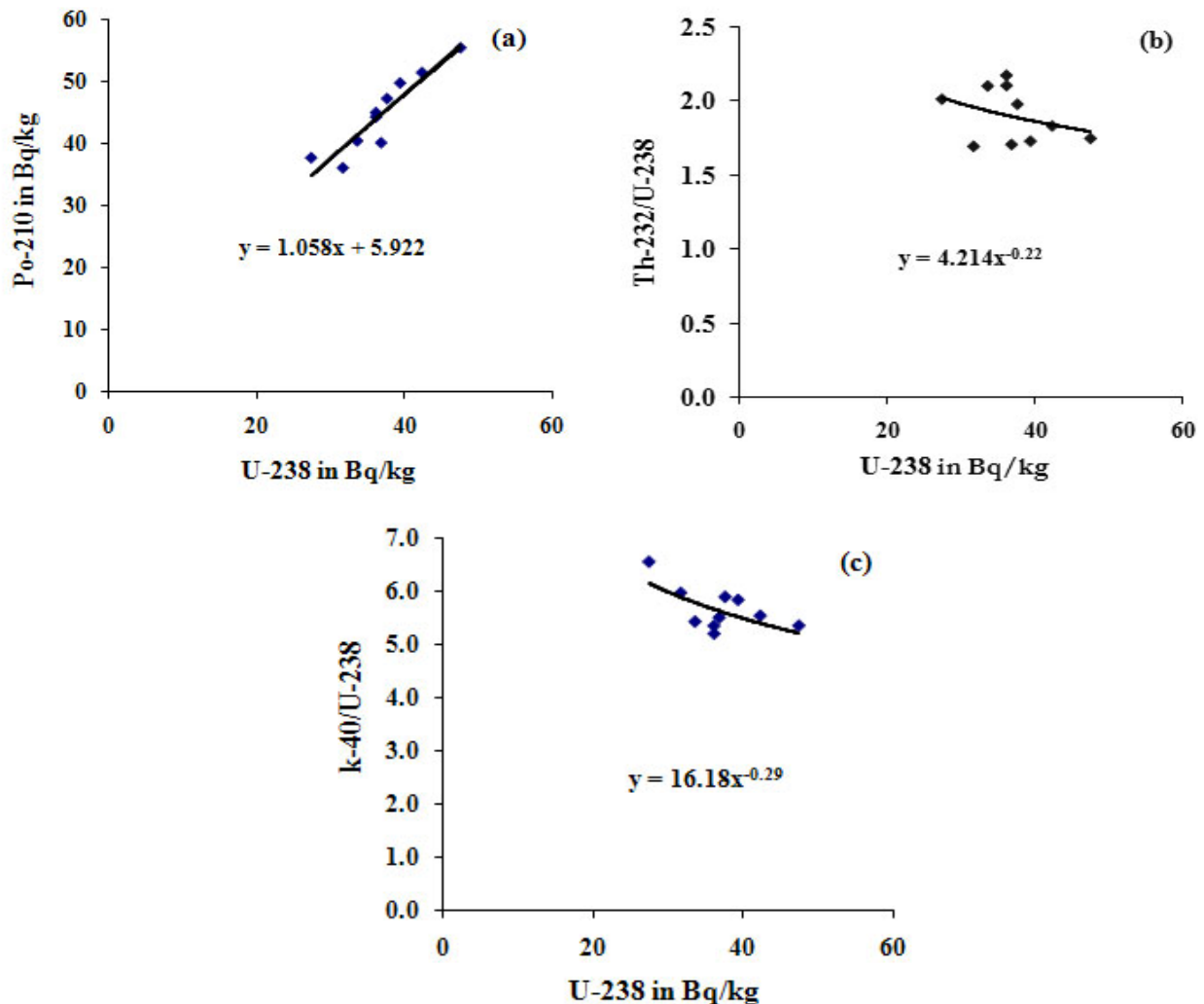
Figure 1. Relation between the activity concentrations of different radionuclides in soil.
