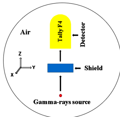
Figure 1. MCNPX simulation geometry (the figure is not in scale).
