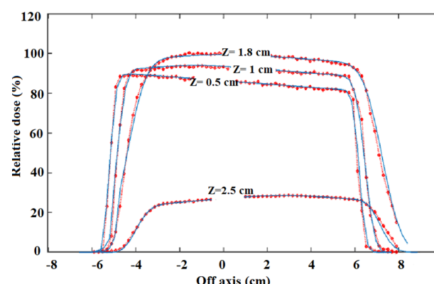
Figure 7. Oblique 10 MeV electron beam profiles at 0.5 cm, 1.0 cm, 1.8 cm, and 2.5 cm depths in the slab phantom; the dotted lines are related to Monte Carlo simulations while solid lines are related to PBA calculations.
