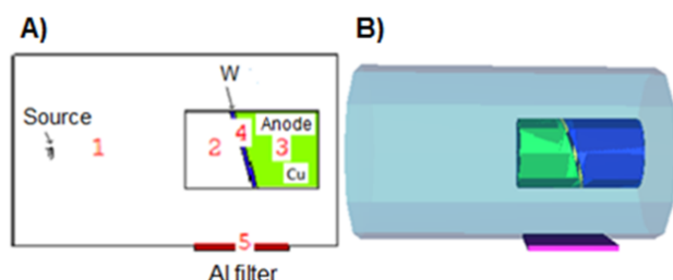
Figure 1. Schematic diagram of the X-ray tube, A) Inside of the tube, B) 3D view of the tube.
