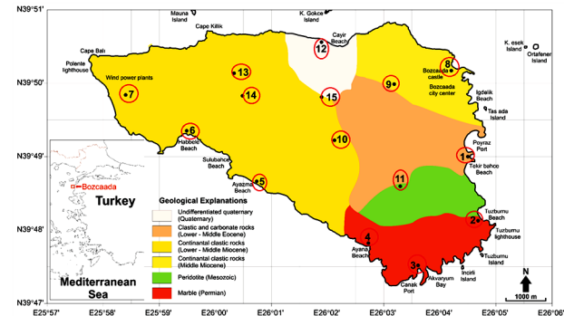
Figure 1. Geological map of Bozcaada Island and the sampling locations ( sampling points are circled in red) (11).
