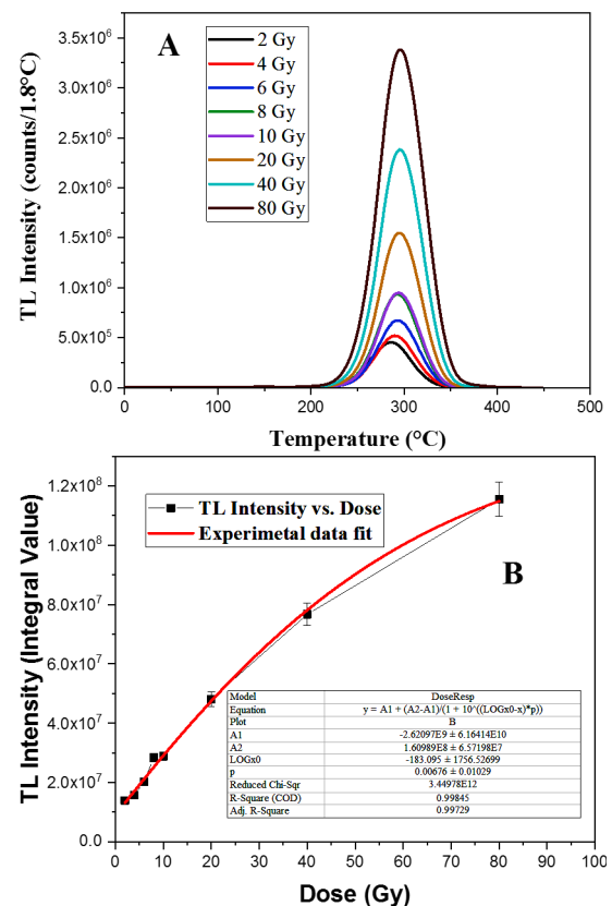
Figure 3. A) TL glow curves for different doses. B) Dose response of TLD-100H. The error bars on TL integral intensities represent the mean \pm SD from three independent experiments.
