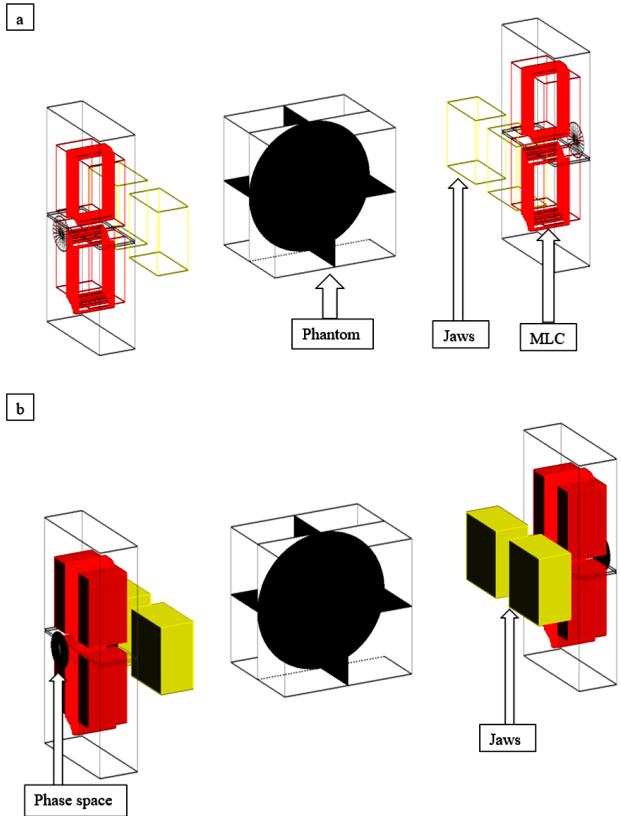
Figure 7. (a, b), Full overview of the linear accelerator with phantom in position for the GATE simulation, where the simulation began with the phase, as photons passed through the multileaf collimator and jaws and were directed towards the phantom in the centre.
