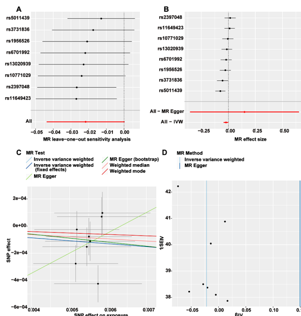
Figure 1. Main Results of the MR Analysis (A. Sensitivity analysis forest plot using the leave-one-out method, changes in effect estimates ( \beta -values) for the remaining SNPs after removing each SNP individually when analyzing the causal effect of exposure factors on radiotherapy sessions; B. Effect Size Analysis, Show the effect size ( \beta -value) of each SNP on radiotherapy sessions in the analysis. The vertical axis is the identifier of the SNP and the horizontal axis is the effect size; C. Causal relationship between SNPs and exposure factors, show the effect size of the association of each SNP on exposure factors and radiotherapy regimen. The horizontal axis is the effect size of the SNP on the exposure factor (SNP effect on exposure) and the vertical axis is the effect size of the SNP on the outcome variable (course of radiotherapy); D. Funnel plot evaluating heterogeneity, comparisons of effect estimates ( \beta -values) and standard errors (SEs) from different Mendelian randomization methods (e.g. Inverse variance weighted, MR Egger) are shown.
