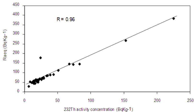
Figure 7. Correlation between R_{aeq} and ^{232}\text{Th} .
