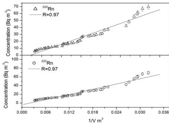
Figure 4. Correlation between 222 Rn and 220 Rn with inverse of the volume of rooms.
