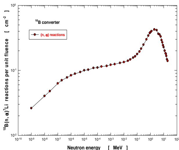
Figure 3. ^{10}\text{B} converter (n, \alpha) response.
