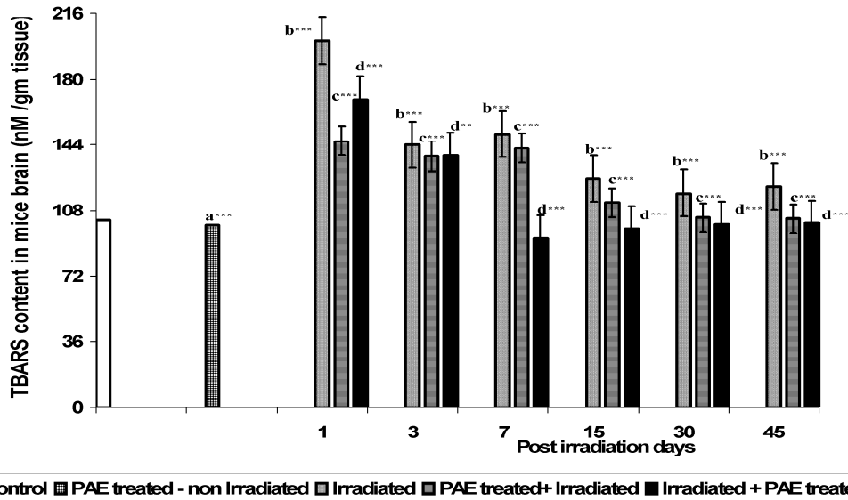
Figure 5. Graph showing protection of lipid peroxidation in mice brain after 5 Gy gamma irradiation by prior and post administration of PAE (methanolic extract of Prunus avium fruits). The lipid peroxidation was measured in terms of nM TBARS/g tissue by LPO assay. Following groups were compared by student's t-test- a: Control v/s PAE treated b: Control v/s Irradiated, c: Irradiated vs PAE treated + Irradiated, d: Irradiated vs Irradiated + PAE treated. Symbols for p values of t-test \leq 0.05 , * <0.01 , ** <0.005 , *** <0.001 , n= non significant.
