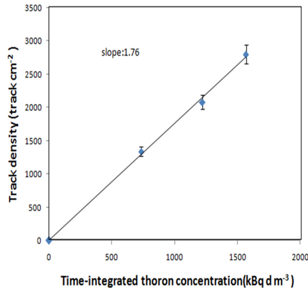
Figure 5. Track density (track per \text{cm}^2 ) for different exposures in thoron measurement by the upper film of the diffusion chamber. (The lower film calibration factor for thoron is zero).
