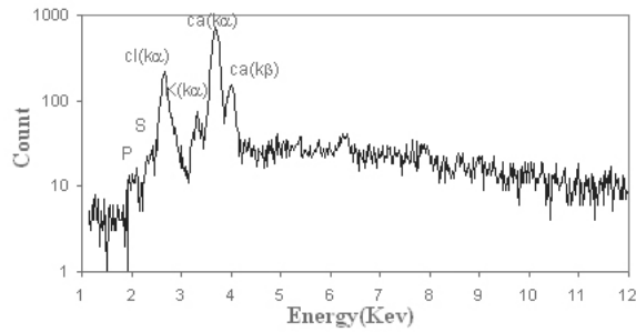
Figure 1. Typical spectra for shell of pigment stones (With a 175 μm Mylar filter).
