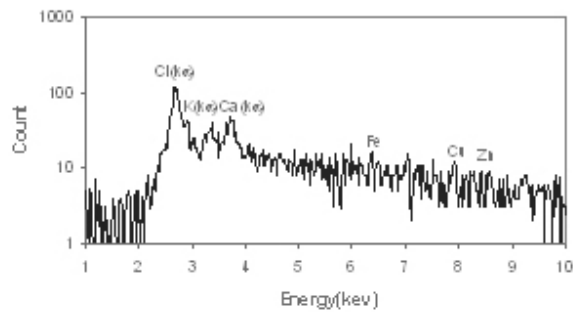
Figure 3. Typical spectra for shell of cholesterol stones (With a 175 μm Mylar filter).
