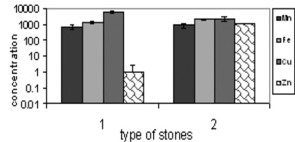
Figure 6. Heavy trace element concentration of gallstones center (Vertical axis 1: Cholesterol stones; Vertical axis 2: Pigment stones).
