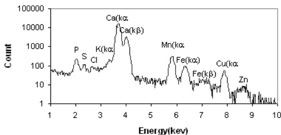
Figure 4. Typical spectra for center of cholesterol stones (With a 175 μm Mylar filter).
