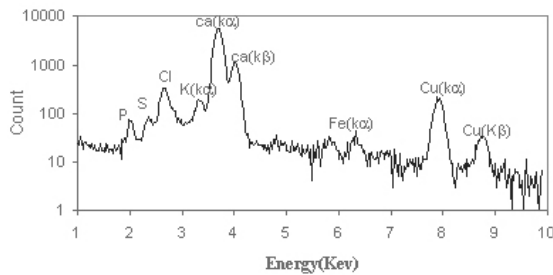
Figure 2. Typical spectra for center of pigment stones (With a 175 μm Mylar filter).
