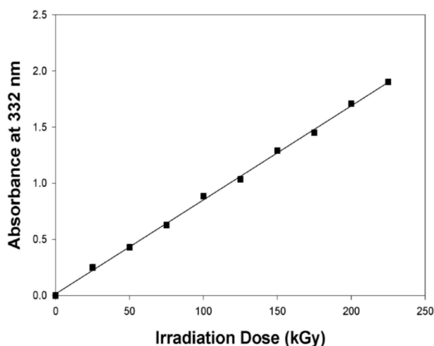
Figure 3. linear regression of the response values at 332 versus the irradiation dose for the concentration 20% of DEF and at dose rate 30 kGy/h.
