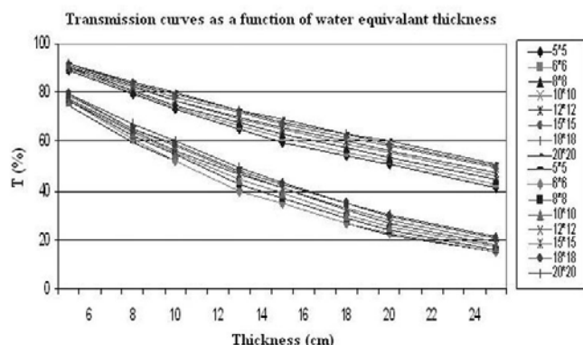
Figure 11. Transmission curves for T and T as a function of water equivalent thickness. T curves are up and T curves are down.
