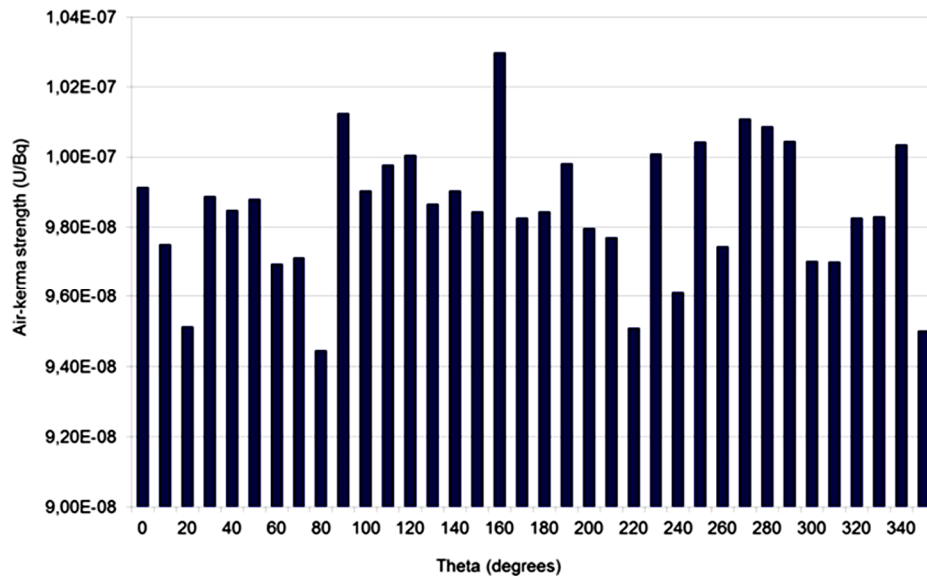
Figure 3. Variation of air kerma rate strength as a function of angle (Theta, \theta ) between the detector and the source center.
