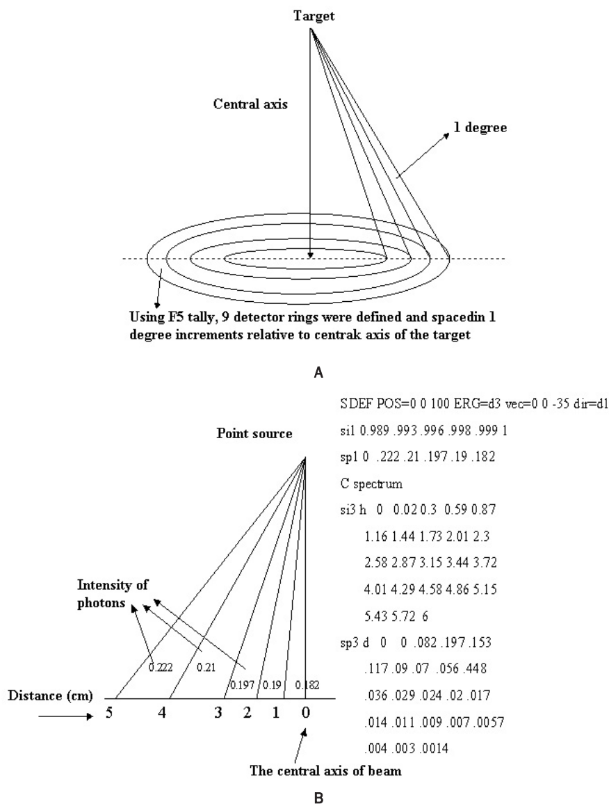
Figure 2. (A) Setup of detectors for scoring the photon fluence, differentiated in energy, angle and intensity. The detector tally plane was located 35 cm downstream from the front surface of the target. (B) This figure illustrates the definition of point source based on calculated photon beam spectra characteristics using ring detectors which is shown in figure (A). The numbers on the right side of part B show a brief definition of source in input file of MCNP4C.
