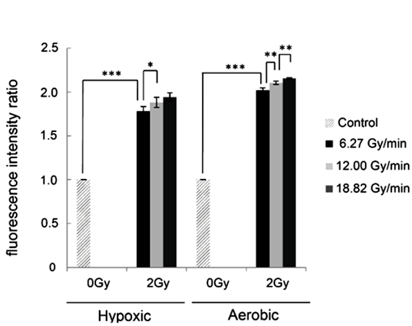
Figure 2. Mean ROS values measured using APF fluorescence shown as a function of dose rate in hypoxic and aerobic cells at 1 h following irradiation at 2 Gy. The error bars represent SD calculated for three independent measurements. *p<0.05, **p<0.01, ***p<0.005
