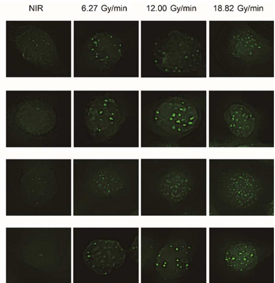
Figure 3. Cell lines under hypoxic and aerobic conditions showing γH2AX foci indicating DNA DSBs with (a) no irradiation (NIR), and 2 Gy irradiation at (b) 6.27 Gy/min, (c) 12.00 Gy/min, and (d) 18.82 Gy/min after 1 h and 24 h of irradiation.
