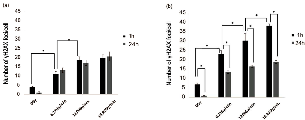
Figure 4. (a) Overall mean number of γH2AX foci following 2 Gy irradiation using 6.27 Gy/min, 12.00 Gy/min, and 18.82 Gy/min at 1 h and 24 h for hypoxic cells. (b) Overall mean number of γH2AX foci following 2 Gy irradiation using 6.27 Gy/min, 12.00 Gy/min, and 18.82 Gy/min at 1 h and 24 h for aerobic cells. The error bars represent SD for three independent measurements. *p<0.05
