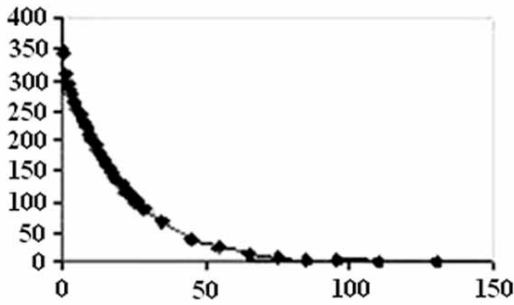
Figure 1. Dose-distance graph of a 100,000 Ci 60 Co linear source.
