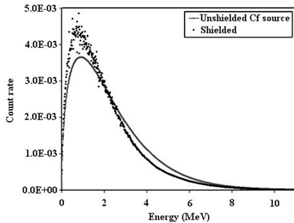
Figure 3. ^{252}\text{Cf} neutron spectrum (per source neutron rate) and the effect of a spherical Pb shield of radius 4 cm on this spectrum.
