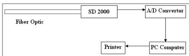
Figure 1. Block diagram of the UV spectrophotometer.
