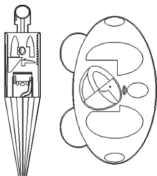
Figure 1. Left: Longitude crosses of ORNL phantom. Right: Transversal cross-sections of an adult female phantom (14) . Heart and lungs are visible in the figure.
