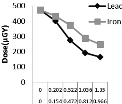
Figure 2. Attenuation of Cs-137 gamma rays as a function of thickness through different shield materials.
