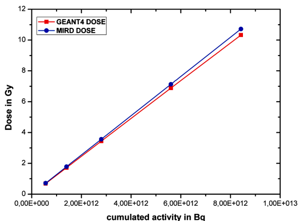
Figure 4. Comparison between MIRD and Geant4: Phantom Case.
