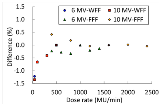
Figure 3. Dose rate dependencies of WFF and FFF beams from 40 to 2400 MU/min. Reference dose rates were 500 MU/min for the WFF beam, 1000 MU/min for the 6 MV FFF, and 1600 MU/min for the 10 MV FFF.
