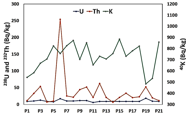
Figure 3. Distribution of Radionuclides in Palar river.
