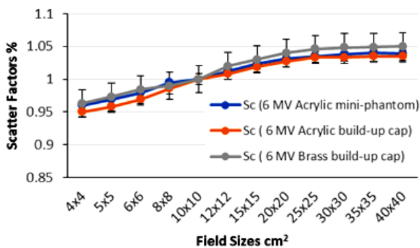
Figure 3. The variation of Collimator Scatter Factors for energy 6 MV with SD in the measurements at different field sizes from 4 × 4 cm 2 to 40 × 40 cm 2 with Acrylic mini-phantom, Acrylic build-up cap and Brass build-up cap.
