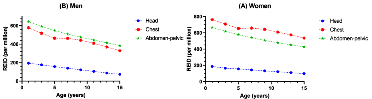
Figure 5. Total number of radiation exposure-induced deaths (REID) per million as an age function for (A) women and (B) men.
