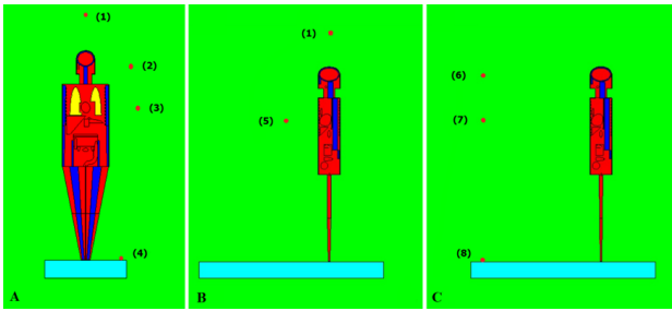
Figure 1. Female MIRD phantom showing the locations of the TLD in both the measurements and simulations a) In the XZ plane, the TLDs were positioned as follows: (1) 0.3 m superior to the head, (2) 0.3 m lateral to the head, (3) 0.3 m lateral to the chest, and (4) 0.3 m lateral to the feet. b) In the YZ plane, the TLDs were situated as follows: (5) 0.3 m anterior to the chest c) In the YZ plane, the TLDs were placed at (6) 1 m anterior to the head, (7) 1 m anterior to the chest, and (8) 1 m anterior to the feet.
