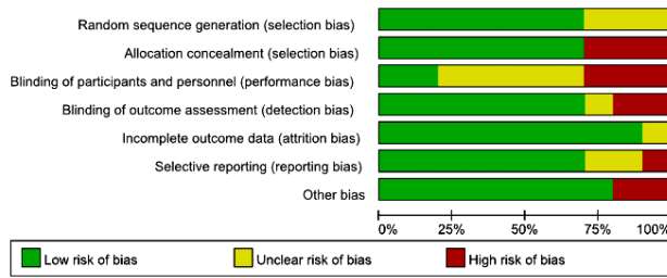
Figure 3. Bar chart for bias risk assessment of the included literatures.
