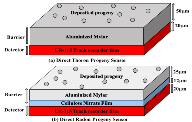
Figure 1. Direct thoron progeny sensor (a) and direct radon progeny sensors (b).
