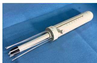
Figure 3. The applicator has nine channels, including one central channel and eight surrounding channels, with a radius of 3.5 cm.
