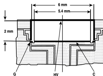
Figure 1. Diagram of a Markus parallel-plate ion chamber.
