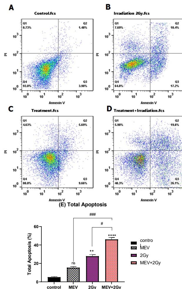
Figure 3. The apoptosis rate of HT-29 cells based on Annexin V/PI staining in (A) control group, (B) irradiation-treated group, (C) MEV group, and (D) MEV+ irradiation group. (E) Percentage of total apoptosis in control, MEV treatment, 2Gy irradiation, and MEV treatment + 2Gy irradiation groups. [ns: not significant, **: p < 0.01, ****: p < 0.0001, compared to the control group] [#: p < 0.05, ###: p < 0.001, compared to single treatment groups].
