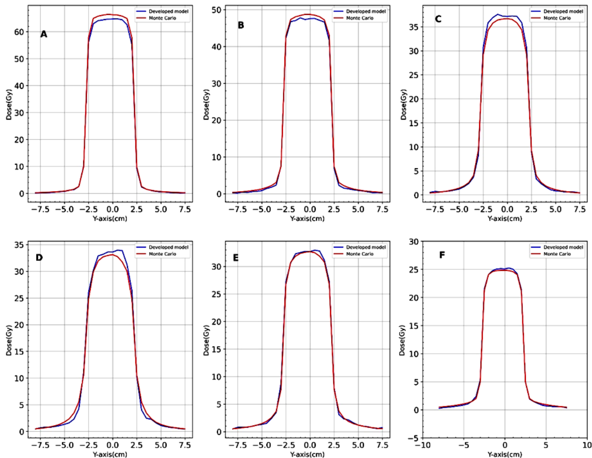
Figure 5. Illustration of the dose profiles in the heterogeneous phantom at various depths from the surface of the phantom. (A) the dose profiles in the water medium at a depth of 5 cm from the surface of the phantom. (B) the dose profiles in the bone heterogeneous region at a depth of 10 cm. (C) the dose profiles at the interface between the bone and lung layers at a depth of 14 cm. (D) the dose profiles at a depth of 16.5 cm within the heterogeneous lung layer. (E) The dose profiles at the interface between the lung and the fourth water layer at a depth of 18 cm. (F) Finally, the dose profiles in the fourth water layer at a depth of 25 cm.
