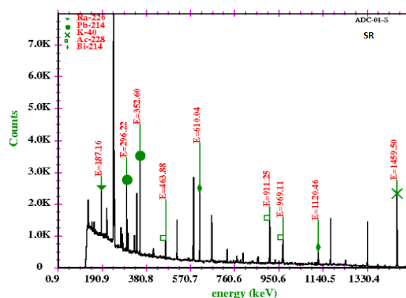
Figure 2 . Spectra of the Stone (SR) sample. Ra-226(\nabla) , Pb-214(\bullet) , K-40(X) , Ac-228(\square) , Bi-214(\blacklozenge)
