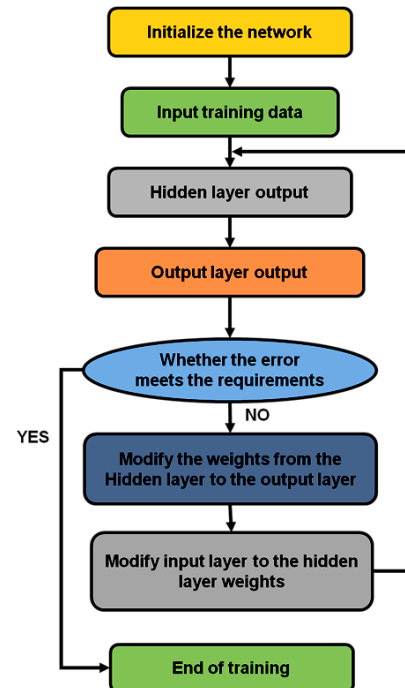
Figure 1. BP neural network learning process.
