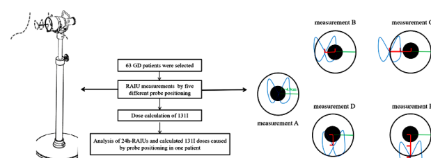
Figure 1. Study flow diagram and 24 hr-radioactive iodine uptake (RAIU) measurement. Left, the thyroid probe uptake system. The neck and thyroid gland are outlined by the dotted line. In the Middle, a schematic depicts the process flowchart of our measurements and calculations in this study. Right, the different placements of the probe. The blue butterfly refers to the shape of a thyroid gland. The black disc refers to the 3.5 cm-diameter NaI crystal. The larger circle surrounding the black disc refers to the collimator with a 9.8cm-diameter scan field. The measurement A is the reference measurement. The green straight line refers to a radius of the collimator, R=4.9 cm. The red line refers to the direction and distance of the probe movements. One red tick mark refers to the movement by 2.5 cm. Two red tick marks refer to the change in probe position by 5 cm.
