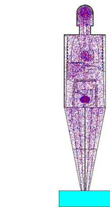
Figure 2. The distribution of ^{18}\text{F-FDG} source in a female MIRD phantom, plotted using VISED. The red points represent electrons, while the blue points represent photons.
