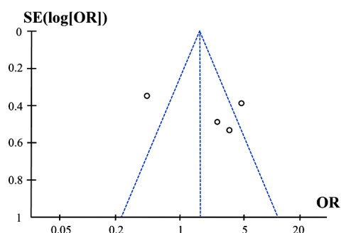
Figure 8. Funnel plot of ORR [The Odds Ratio (OR) is used to measure the association between two groups, representing the relative magnitude of risk ratio or effect size. SE(\log[OR]) is the logarithm of the standard error of OR. Standard error is a measure used to assess the difference between the sample estimate and the population parameter. Taking the logarithm of OR and calculating its standard error aims to better express the precision and credibility of OR. A smaller value of SE(\log[OR]) indicates a more precise estimate of OR and a narrower confidence interval.]
