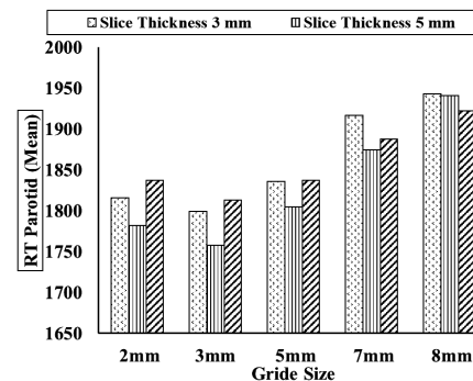
Figure 8. Variation of RT Parotid with slice thickness 3,5,7 mm as a function in different grid sizes using VMAT technique.
