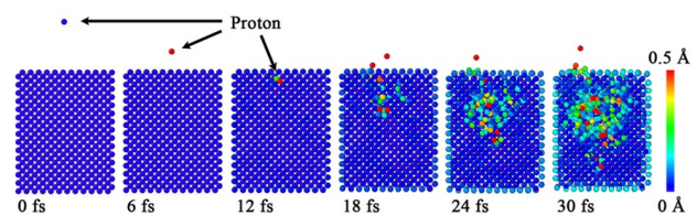
Figure 3. Entire The entire damage process of Ti-12Mo-6Zr-2Fe alloy (coloured by atomic displacements).
