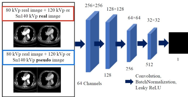
Figure 3. Pix2pix model comprises discriminator Patch GAN.
