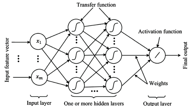
Figure 4. An architecture of multi-layer perceptron (MLP) model. This figure demonstrates the architecture of the Multi-Layer Perceptron (MLP) model, a deep learning approach used in gastric cancer recurrence prediction. The diagram shows the multiple layers of neurons in the MLP, highlighting how data flows through the network and how hidden layers learn complex patterns in the data. The figure is key in illustrating how MLP models handle non-linear relationships between clinical, genomic, and imaging data for gastric cancer prediction.
